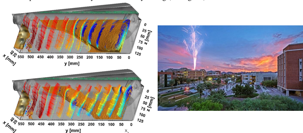
PIV of baseline (top) and controlled (bottom) flow over the deflected flap of a finite wing.
